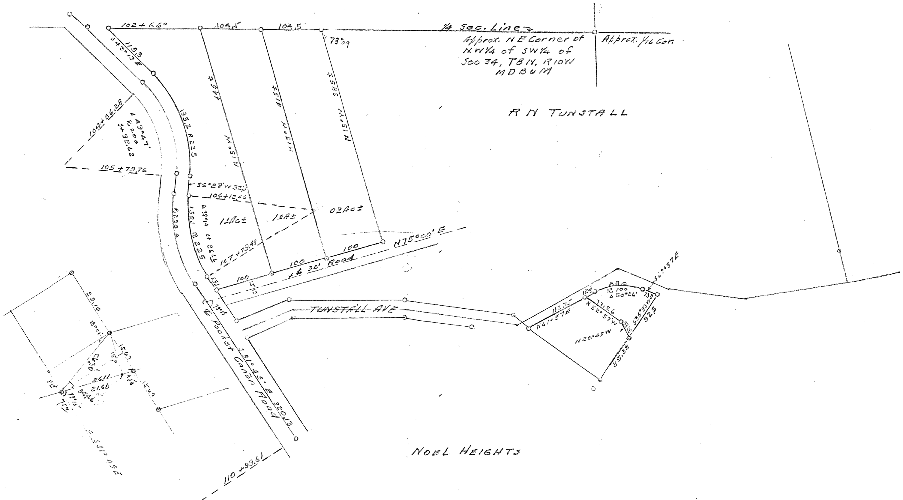
-sketch- Location of Proposed Small parcels in R.H. Corner of lands of R H Tunstall Scale 1" = 100' April 1943 G.S. Abbott.
